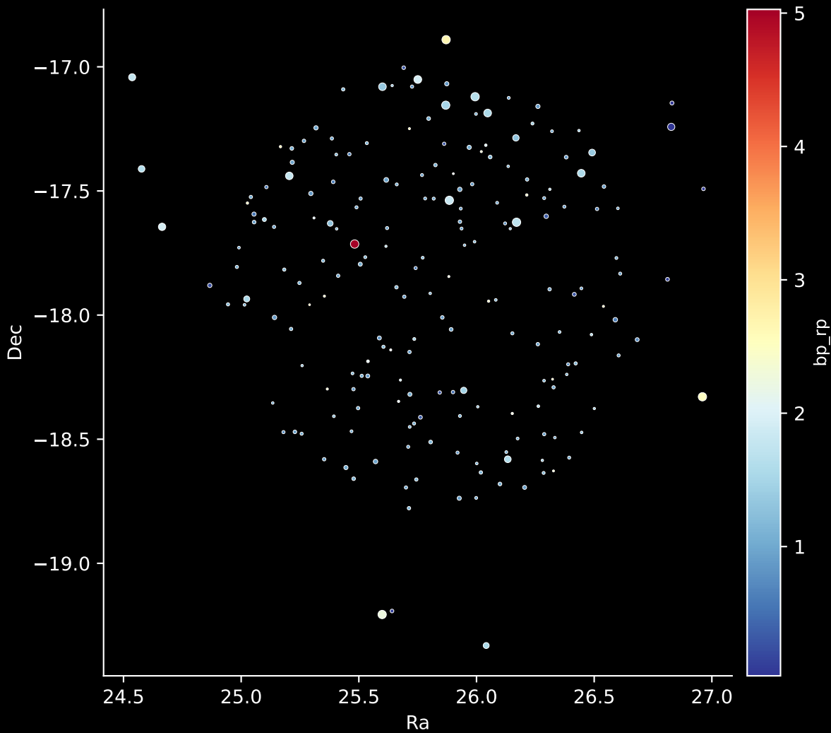
APOGEE DR17 Field: [K2_C7_018-11_btx] Stars: 199
