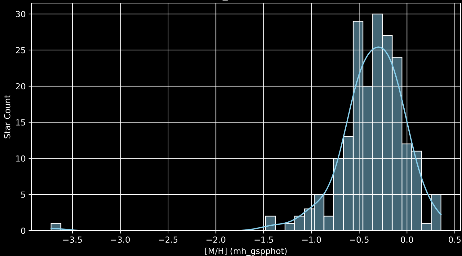
APOGEE DR17 Field: [K2_C7_018-11_btx [M/H] (mh_gspphot) (n= 198)
