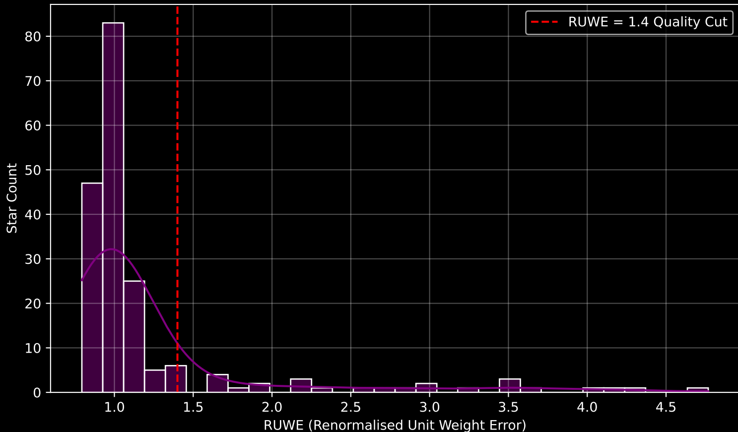
GAPOGEE DR17 Field [K2_C7_018-11_btx] RUWE Distribution (n= 191)
