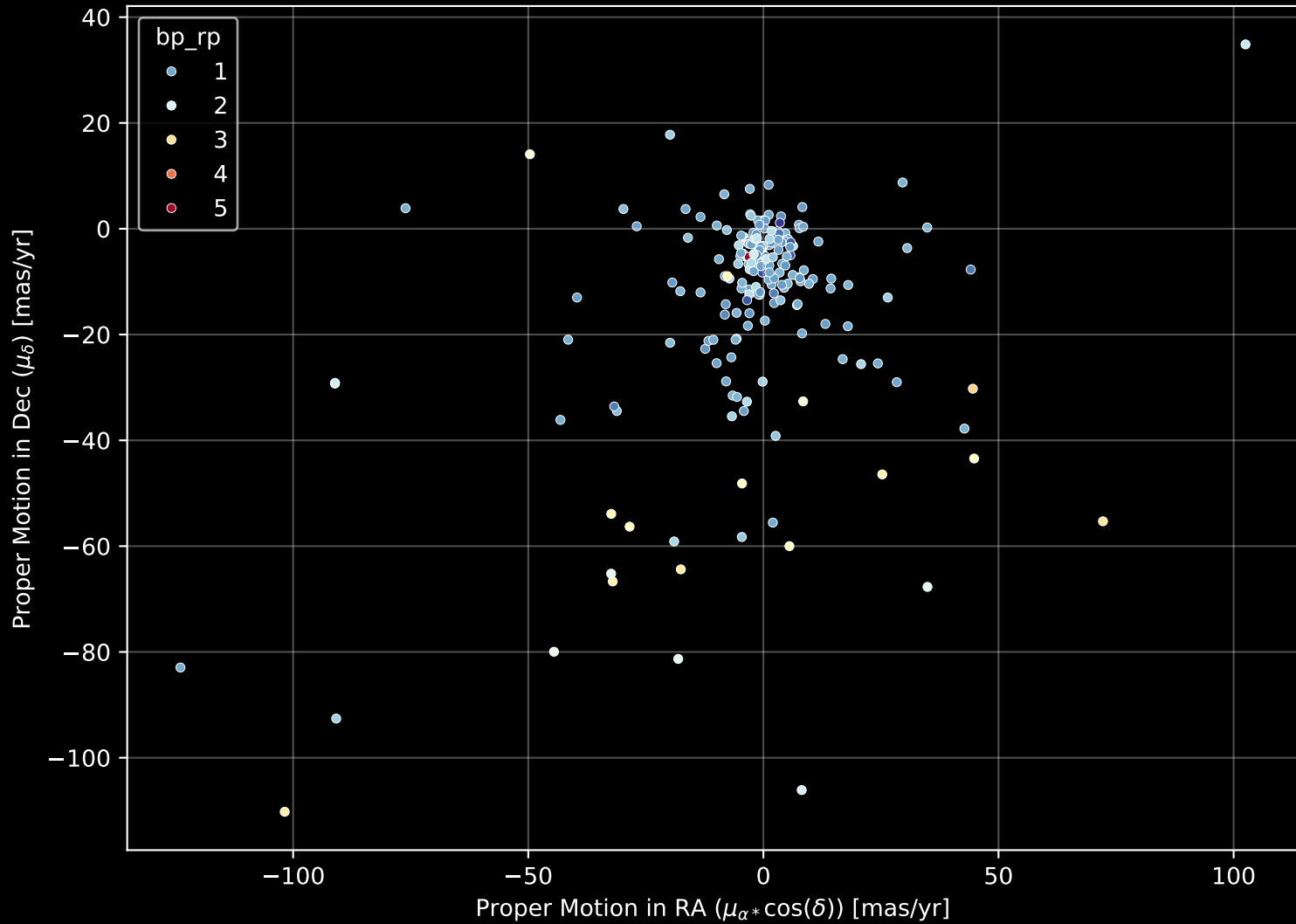
APOGEE DR17 Field: [K2_C7_018-11_btx] Proper Motion Diagram (n= 199)
