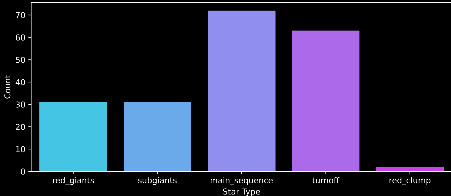
APOGEE DR17 Field: [K2_C7_018-11_btx] Count plot of Star Type
