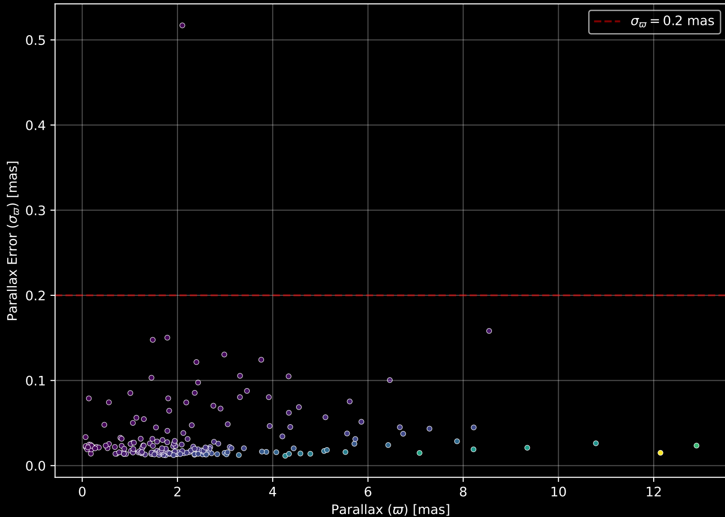
APOGEE DR17 Field: [K2_C7_018-11_btx] Parallax Quality (n= 199)
